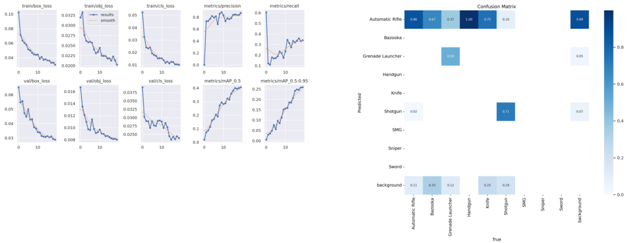
(a) YOLOv8 Training Curves
